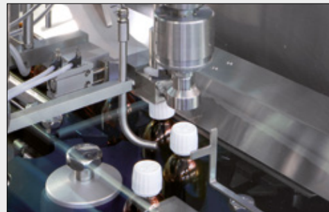
Intermittent motion capping machine
