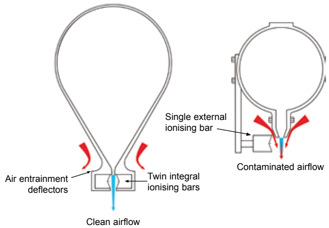
JetStream Air Knife
