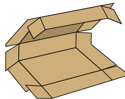
FEFCO STYLE 0409 Five panel wrap.
