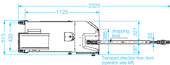
Layout Sonixs MS-6 KR (850 mm x 1400 mm)
